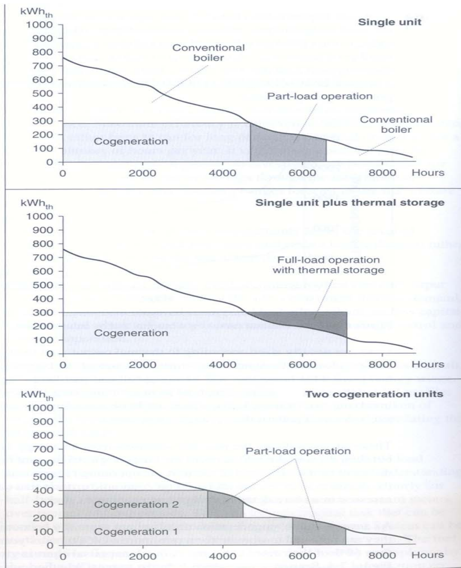
Thermal load duration curve for a hospital: a) for a single 300 kW th cogeneration unit; b) for the same unit with thermal storage; c) for two 200 kW th cogeneration units.
